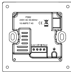
Fig.2 Back View
